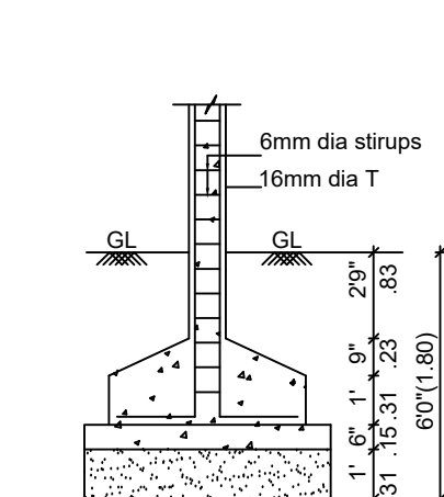
COLUMN FOUNDATION DETAIL
