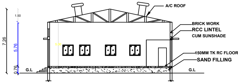
SECTION ON SS
