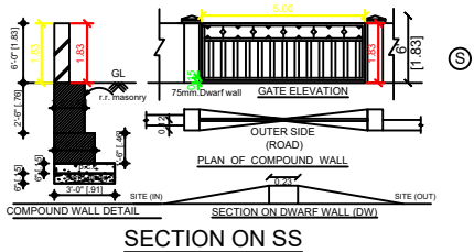
SECTION ON SS
