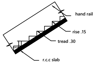
STAIR
