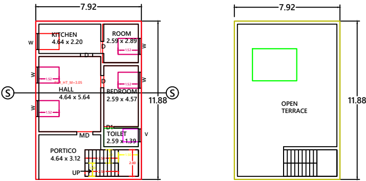
GROUND FLOOR
