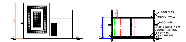
ELEVATION SECTION ON X-X
