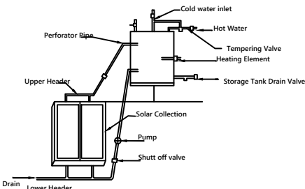
SOLAR HEATER DEATIL
