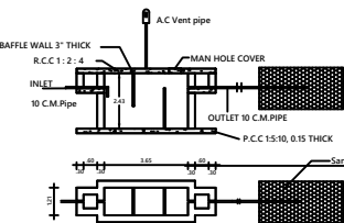
SEPTIC TANK DETAIL
