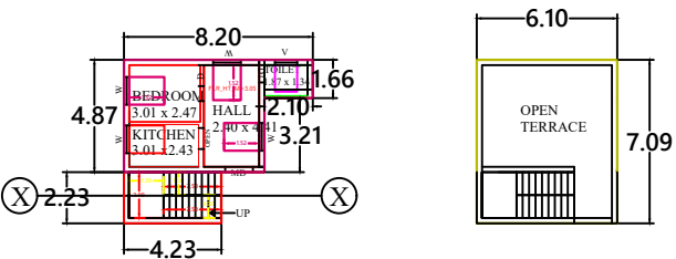
GROUND FLOOR PLAN TERRACE FLOOR PLAN
