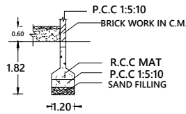
FOUNDATION DEATIL
