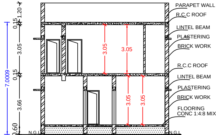
CROSS SECTION "SS"
