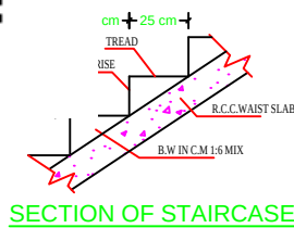
SECTION OF STAIRCASE
