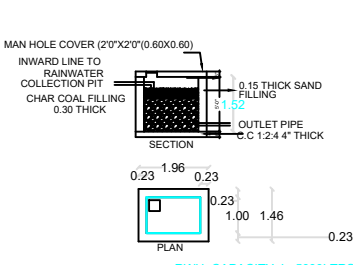
DETAILS OF RAINWATER HARVESTING
