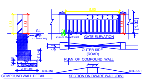
DETAILS OF COMPOUND WALL
