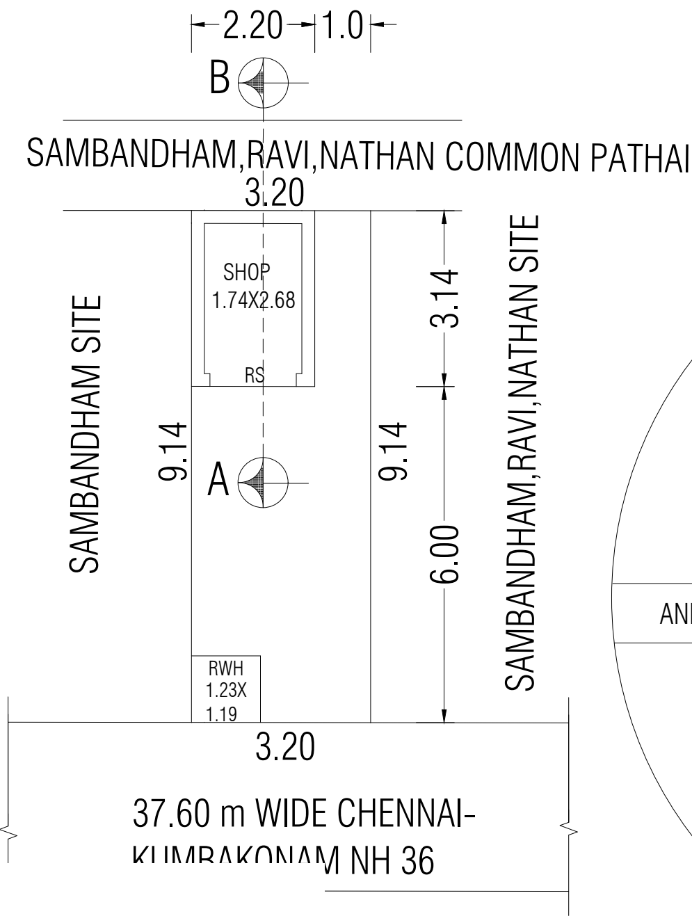
FLOOR PLAN
