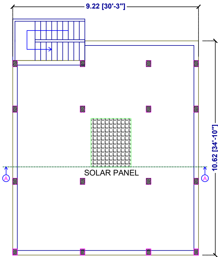
TERRACE PLAN
