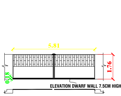
GATE ELEVATION
