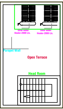
FIRST FLOOR PLAN HEAD ROOM
