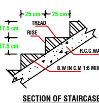
SECTION OF STAIRCASE
