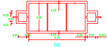
PLAN & SECTION OF SEPTIC TANK & DISPERSION TRENCH
