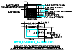
DETAILS OF COLLECTION SUMP FOR RAIN WATER HARVESTING OF ROOF TOP RUN WATER
