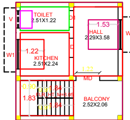
PRO.FIRST FLOOR PLAN
