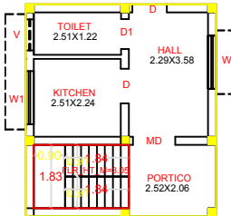
EX.GROUND FLOOR PLAN
