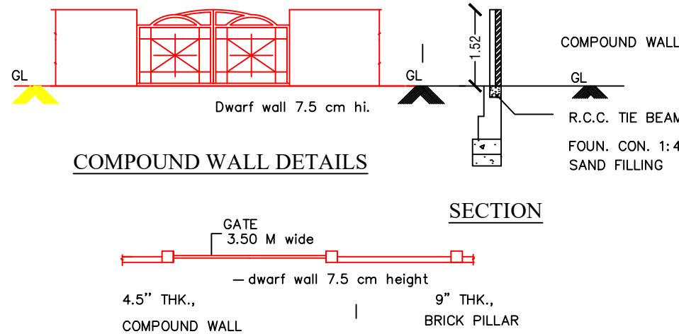
COMPOUND WALL PLAN
