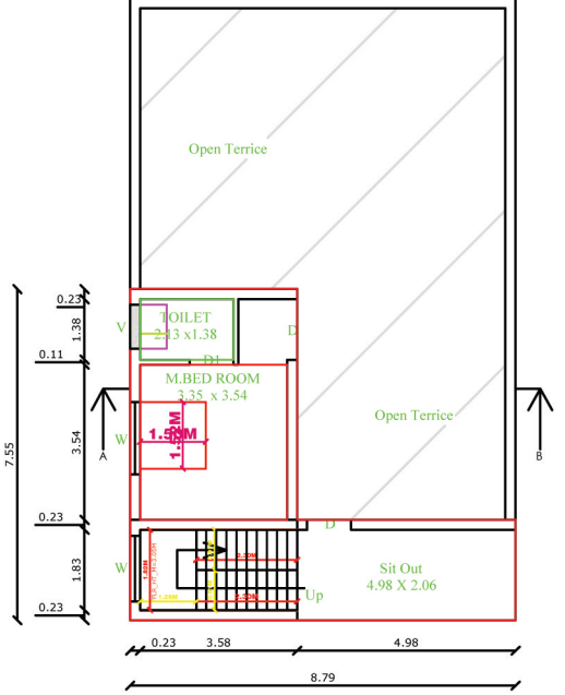
FLOOR-01
