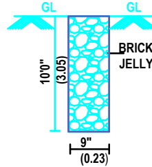
PERCOLATION PIT
