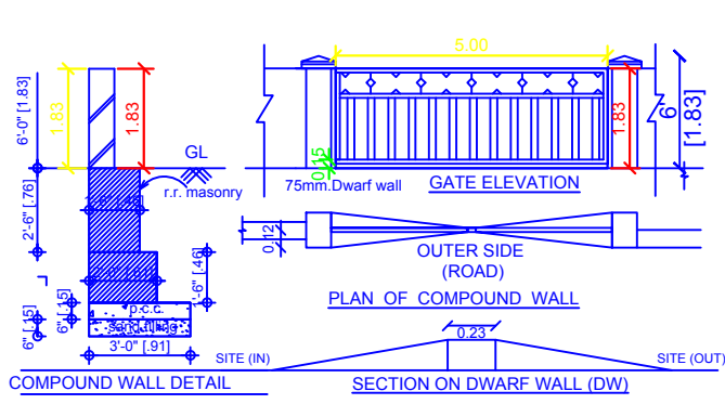
DETAILS OF COMPOUND WALL
