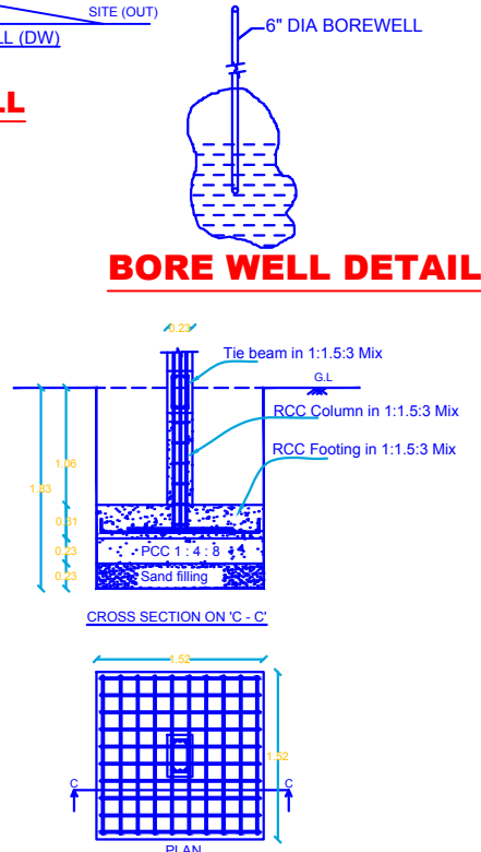
COLOUMN FOUNDATION DETAILS
