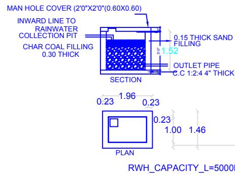
DETAILS OF RAINWATER HARVESTING
