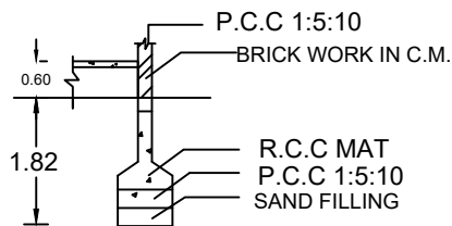
FOUNDATION DETAILS
