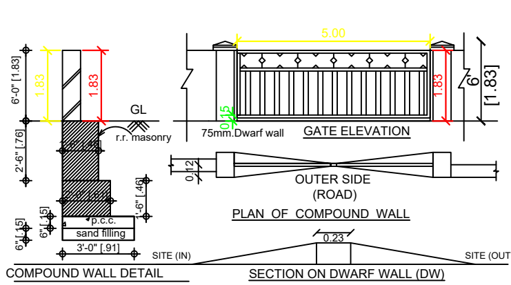
FRONT ELEVATION
