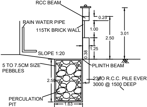
RAINWATER HARVESTING
