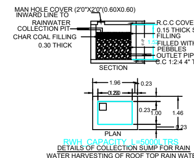
RAINWATER HARVESTING
