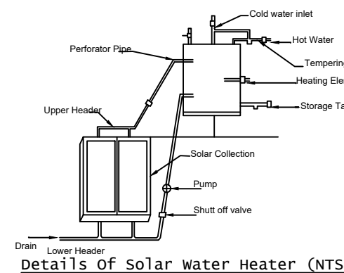
Details of Solar Water Heater (NTS)
