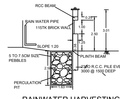
RAINWATER HARVESTING
