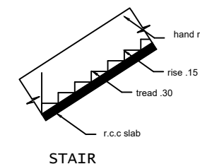
STAIR
