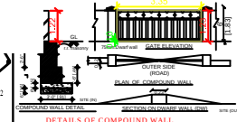
DETAILS OF COMPOUND WALL
