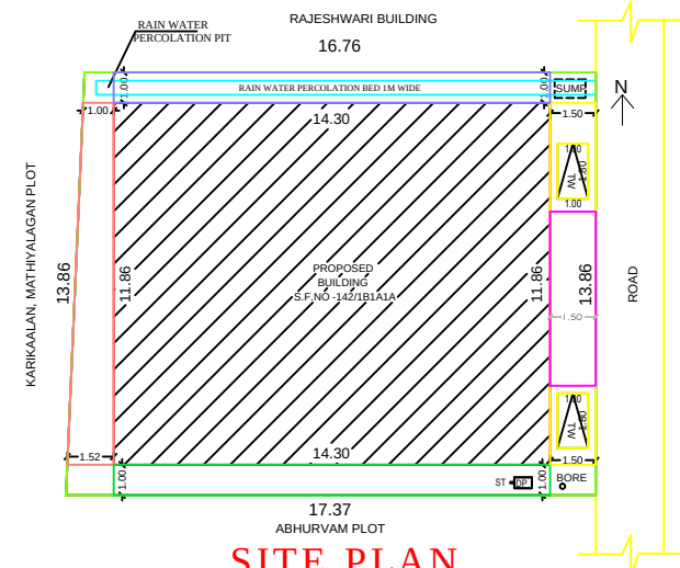
SITE PLAN
