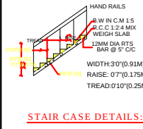
STAIR CASE DETAILS:-
