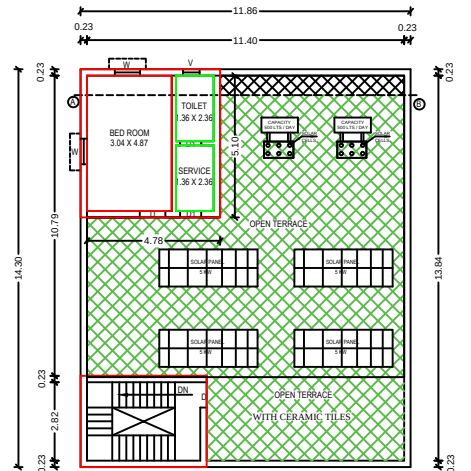
PROPOSED SECOND FLOOR PLAN
