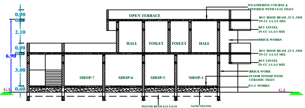
SECTION ON 'X - X'
