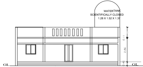
FRONT ELEVATION EAST FACING.
