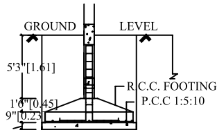
FOUNDATION DETAILS SECTION
