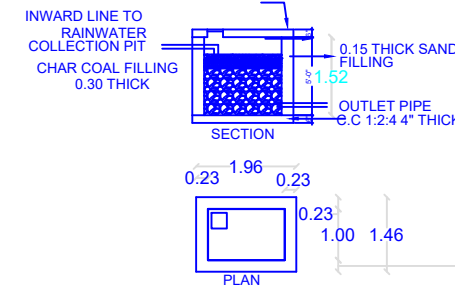
DETAILS OF RAINWATER HARVESTING
