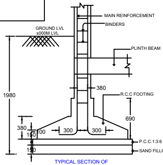
TYPICAL SECTION OF R.C.C COLUMN FOUNDATION
