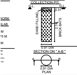
DETAILED PLAN OF RAIN WATER COLLECTION AND STORAGE
