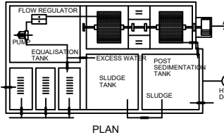
PLAN SEWAGE TREATMENT PLANT DETAILS WASTE WATER RECYCLING UNIT
