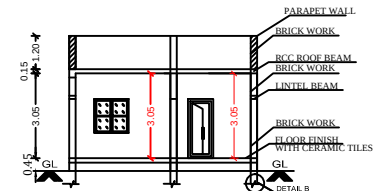
SECTION ON AB
