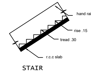
STAIR
