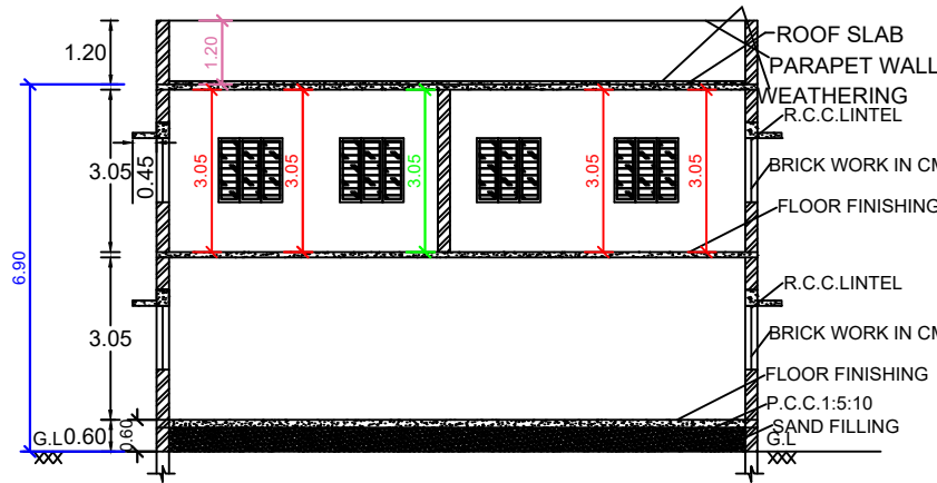
SECTION ON SS
