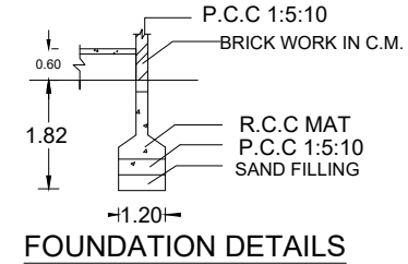
FOUNDATION DETAILS
