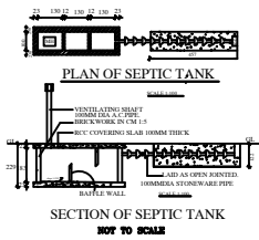
SECTION OF SEPTIC TANK
