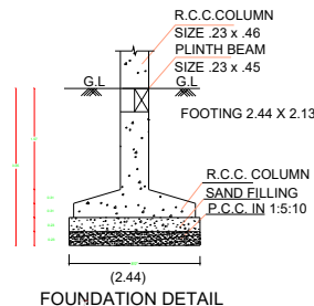
FOUNDATION DETAIL
