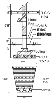
TRIAL PIT FOR FOUNDATION SCALE 1:25 DIMENSION ARE IN MM
