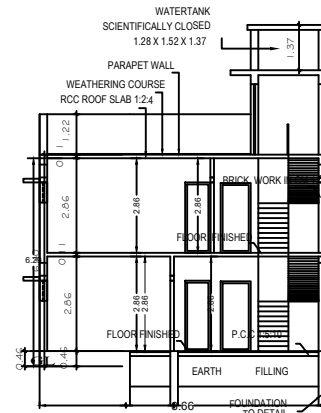
SECTION "A-B"
