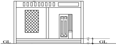
FRONT ELEVATION SOUTH FACING.
