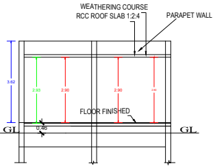
SECTION "A-B"
