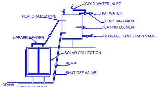
DETAILS OF SOLAR WATER HARVESTING (NTS)
