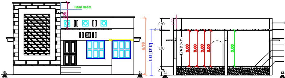
FRONT ELEVATION
