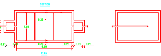
PLAN & SECTION OF SEPTIC TANK & DISPERSION TRENCH
