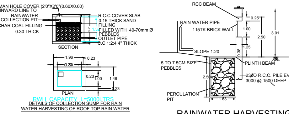
RAINWATER HARVESTING
