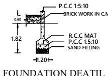
FOUNDATION DEATIL
