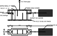
SEPTIC TANK DETAIL
