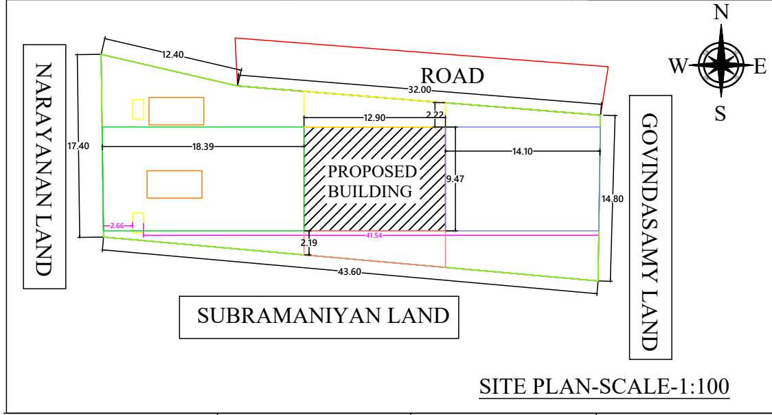
PROPOSED SITE: SF.NO:189/8A1A
