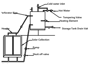
SOLAR HEATER DEATIL
