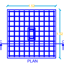
COLOUMN FOUNDATION DETAILS
