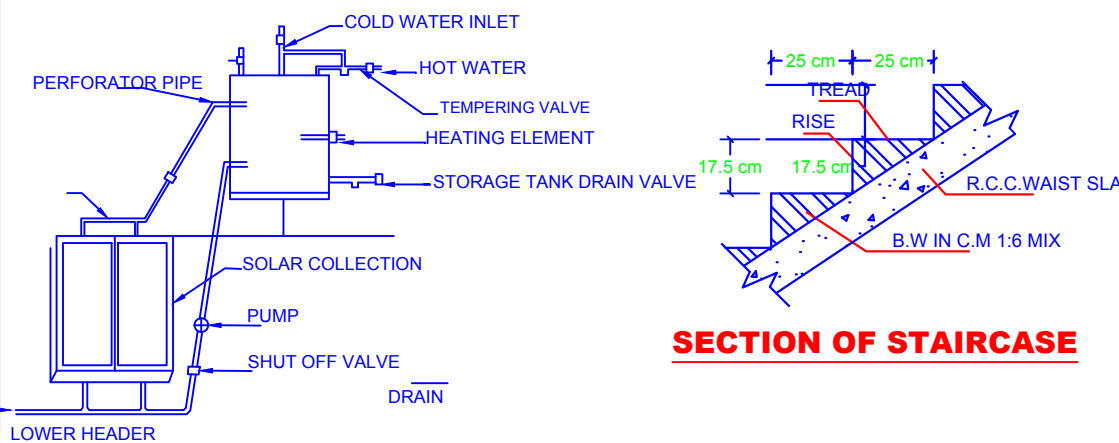
DETAILS OF SOLAR WATER HARVESTING (NTS)
