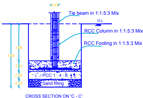
CROSS SECTION ON 'G-C'
