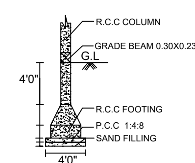
COLOUMN FOUNDATION DETAILS
