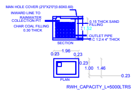
DETAILS OF RAINWATER HARVESTING
