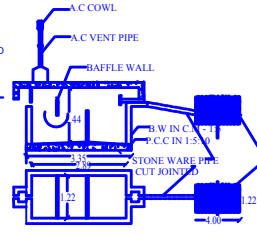
SEPTIC TANK DETAILS
