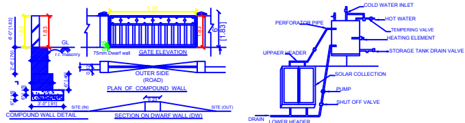
DETAILS OF COMPOUND WALL
