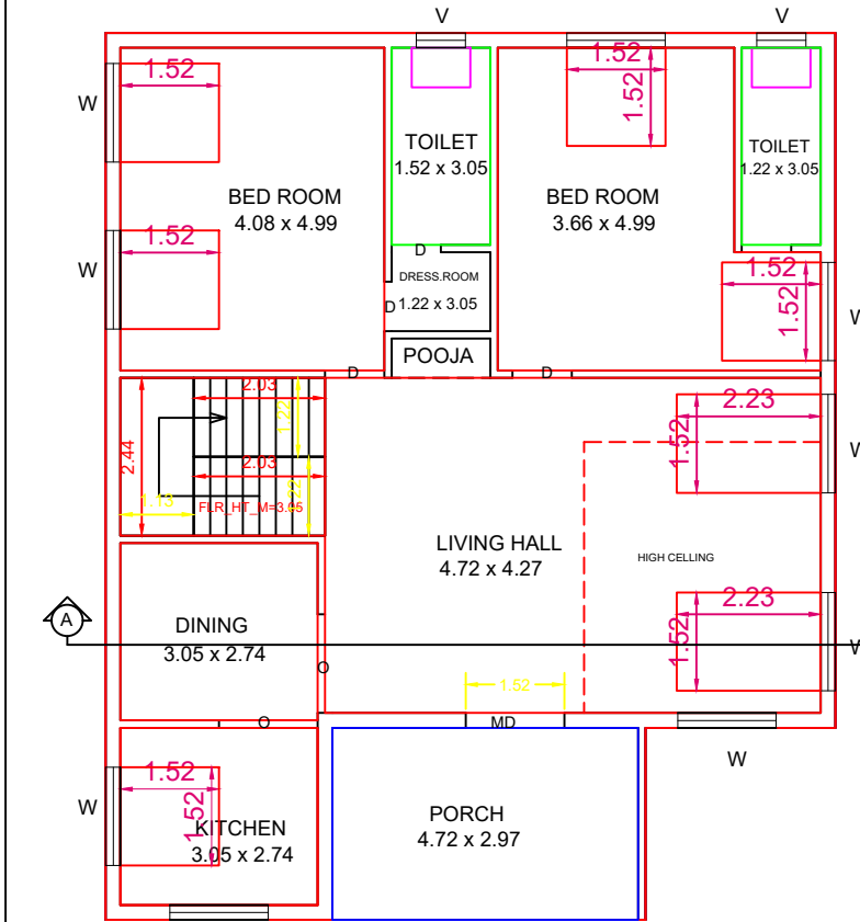
PRO.GOUND FLOOR PLAN
