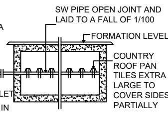
SECTION OF DISPERSION TRENCH
