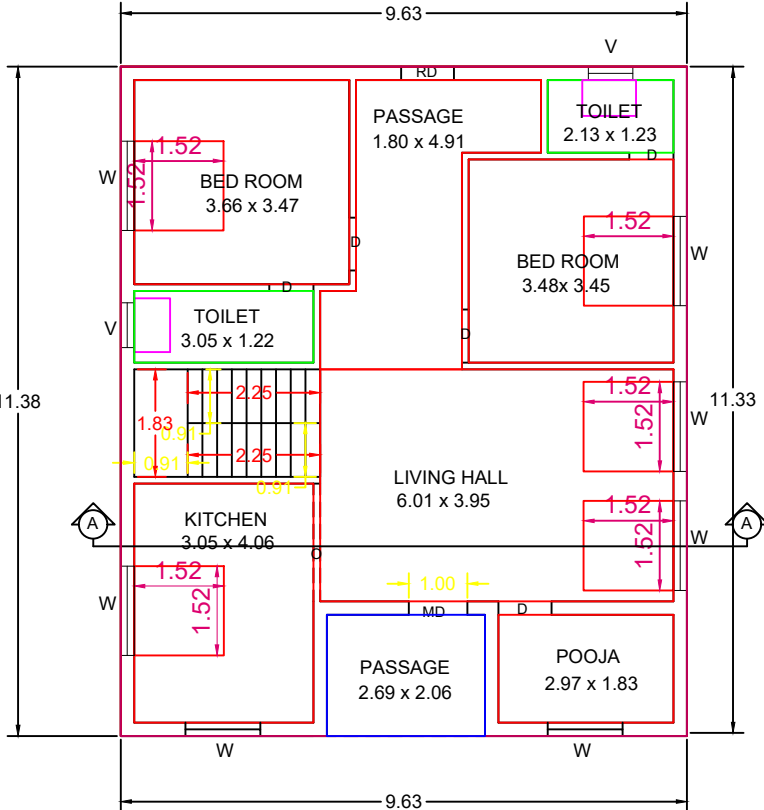
PRO.GOUND FLOOR PLAN
