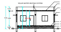
SECTION ON MM
