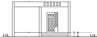
FRONT ELEVATION SOUTH FACING.
