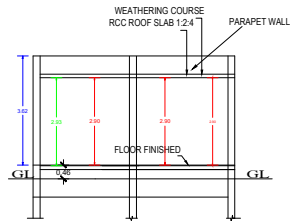
SECTION "A-B"
