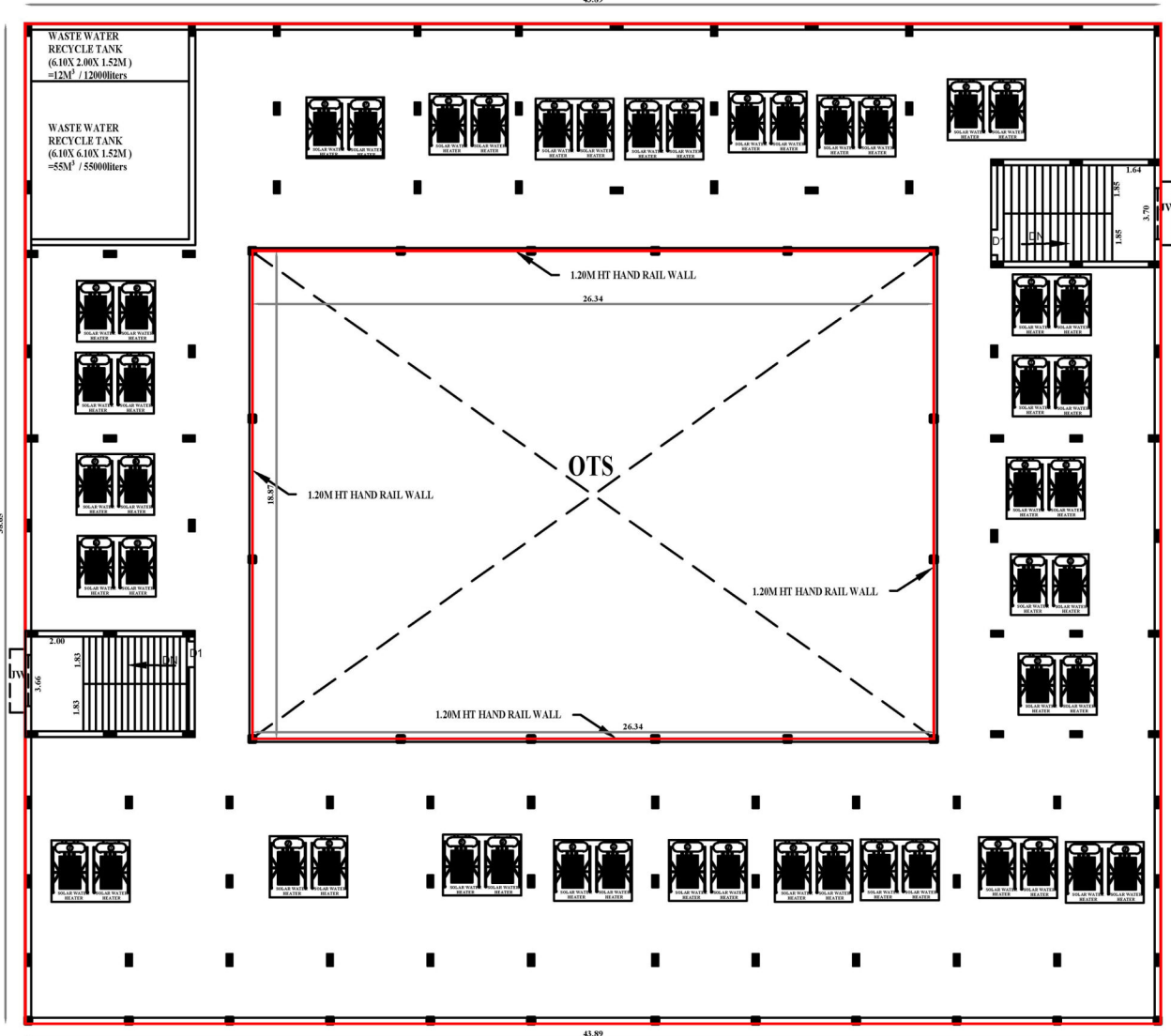
OPEN TERRACE FLOOR PLAN
