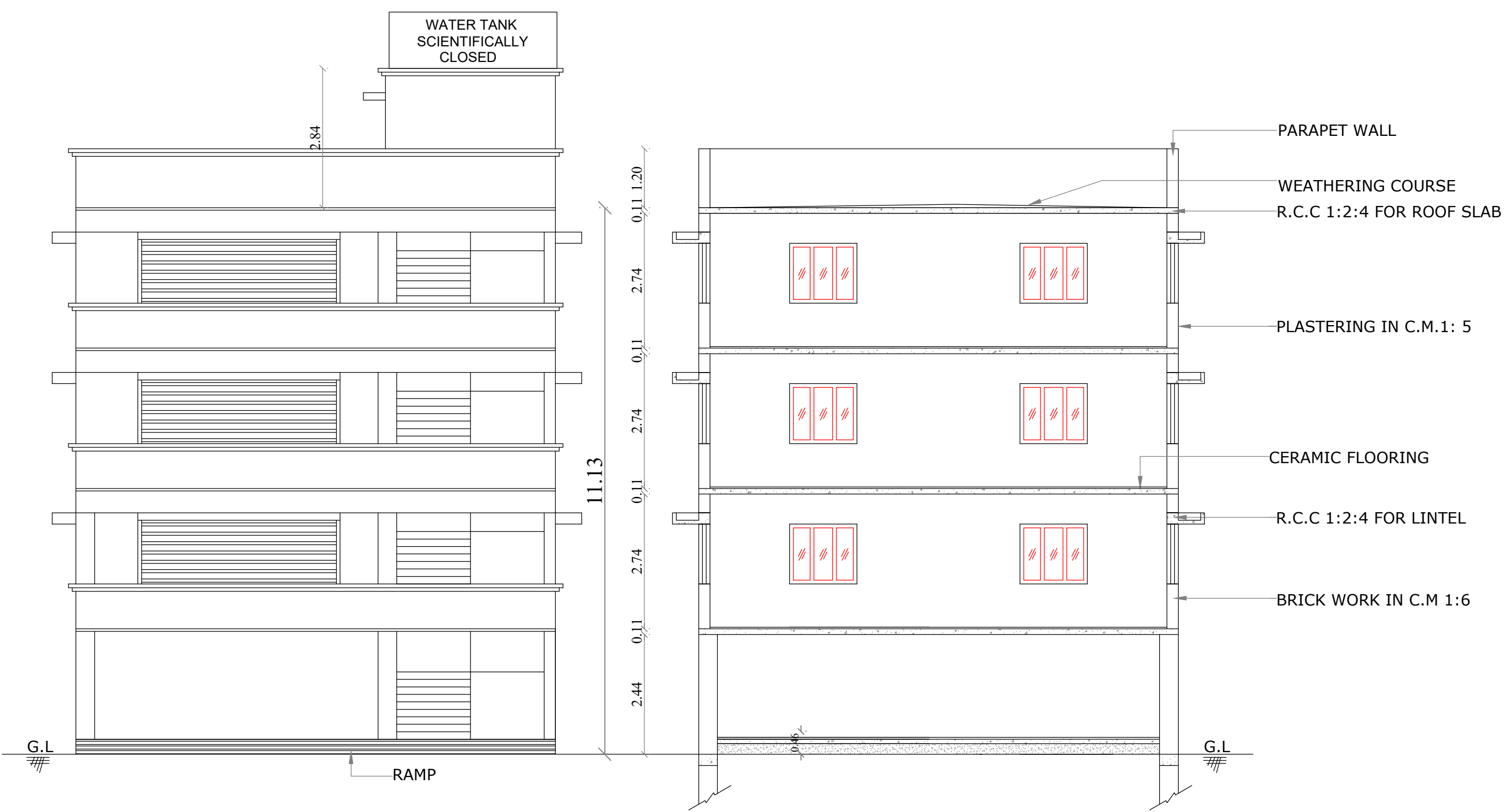
FRONT ELEVATION
