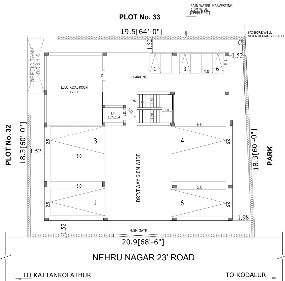
SITE PLAN
