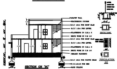
SECTION ON 'SC'
