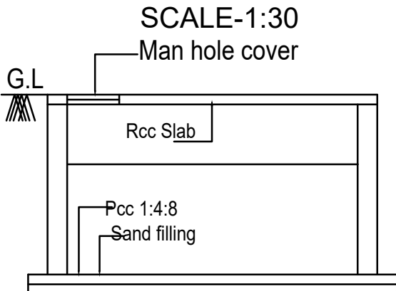
Section 'C-C'
