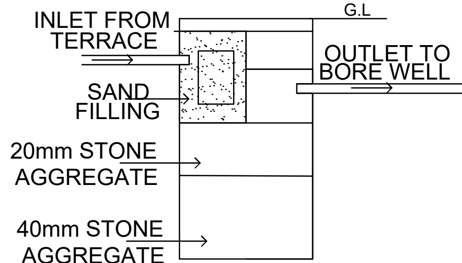
SECTION OF RAIN WATER HARVESTING DETAIL
