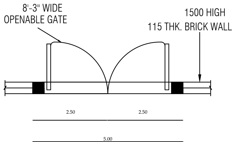
PLAN COMPOUND WALL DETAIL
