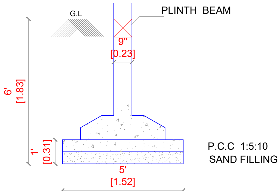
FOUNDATION DETAIL
