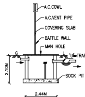
SEPTIC TANK
