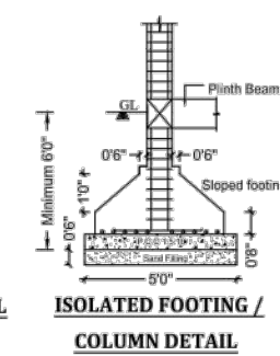
COLUMN DETAIL
