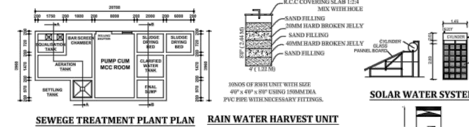
SEWEGE TREATMENT PLANT PLAN RAIN WATER HARVEST UNIT
