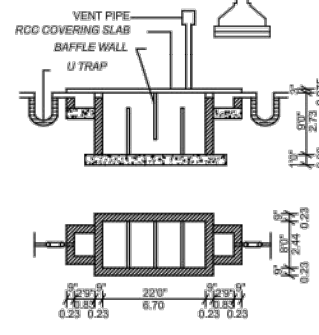
SEPTIC TANK WITH U TRAP
