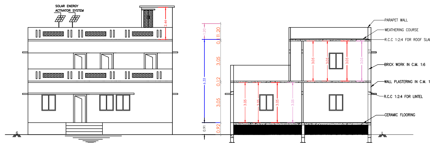
FRONT ELEVATION
