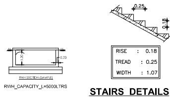
STAIRS DETAILS
